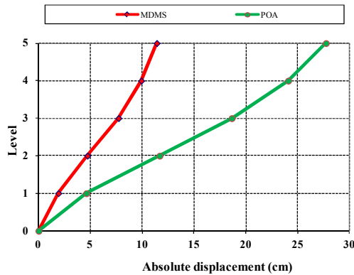
Figure 5: Absolute displacement for longitudinal direction XX
